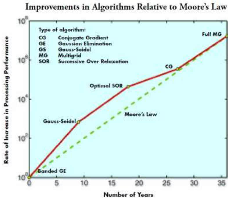
Figure 1. The relative gains in some algorithms for the solution of an electrostatic potential equation on a uniform cubic grid compared to improvements in the hardware (Moore's Law).
